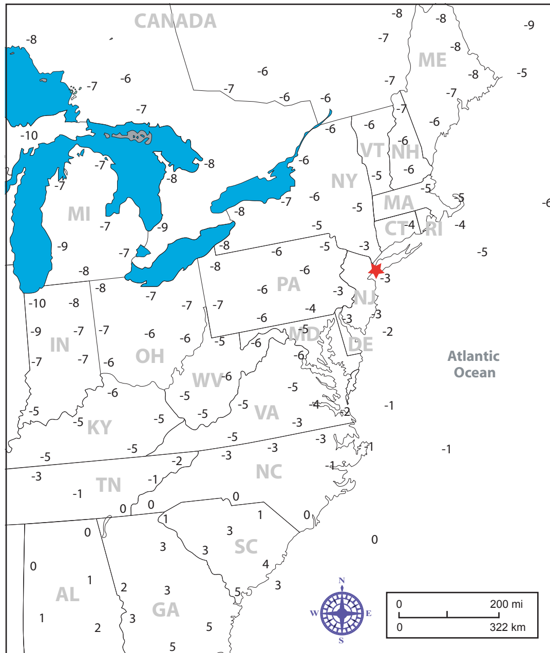
850mb Temperature (°C) Day 2 Analysis for 12Z 29 DEC 00
