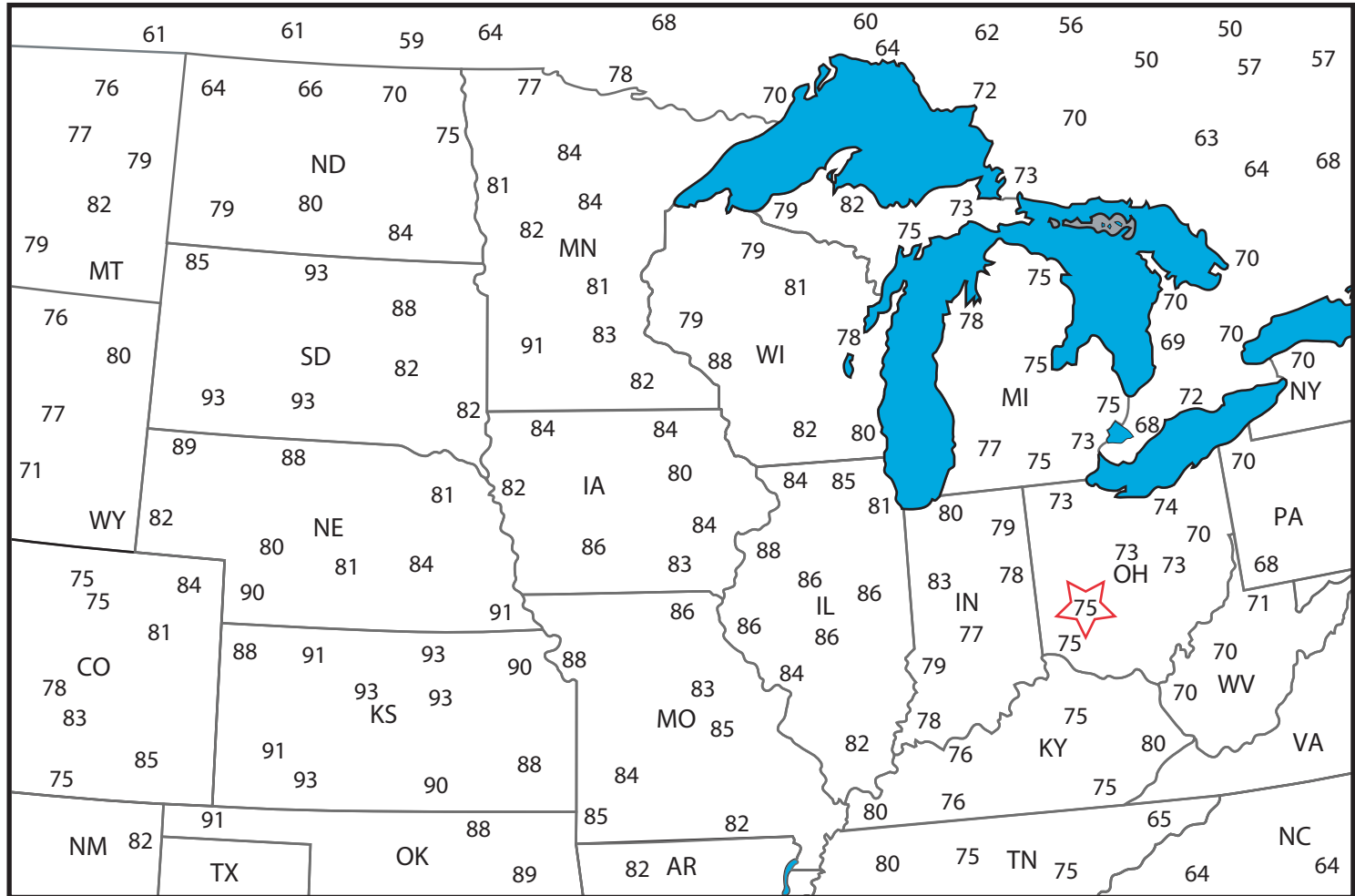
Surface Temperature (°F) Day 2 Analysis for 18Z 18 SEP 00
