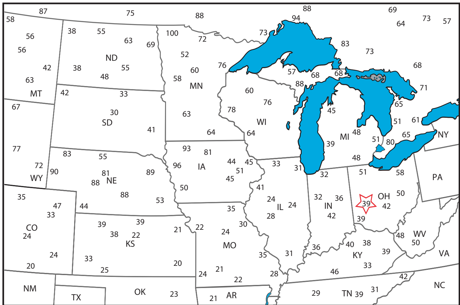
Surface Relative Humidity (%) Day3 Analysis for 18Z 19 SEP 00
