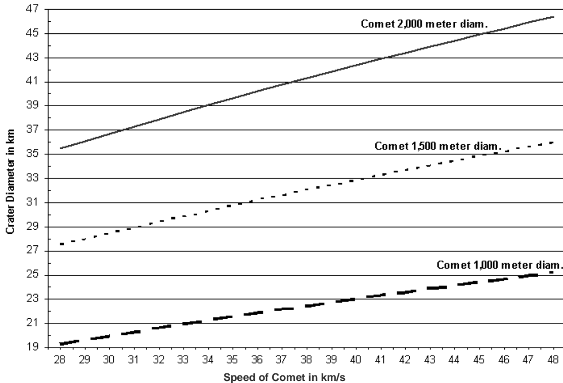
Graph 2: Crater Diameter
